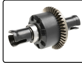
C-00180-687 Diff Assembly - Front / Rear - 43T Bevel Gear - 20K Oil Filled - 1 Set
